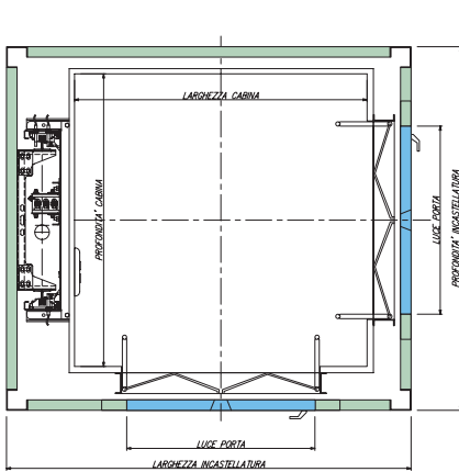
Due accessi adiacenti Double entrances nearby
