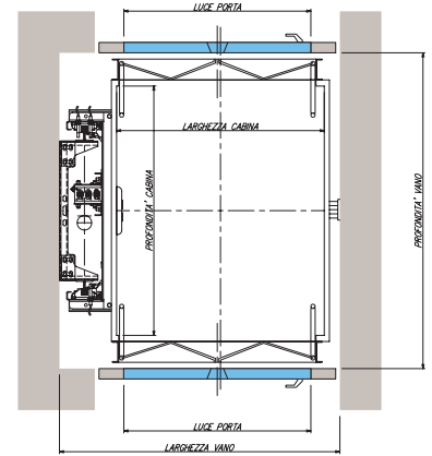
Due accessi opposti Double entrances opposed
