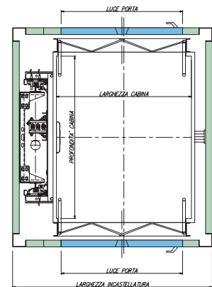
Due accessi opposti Double entrances opposed
